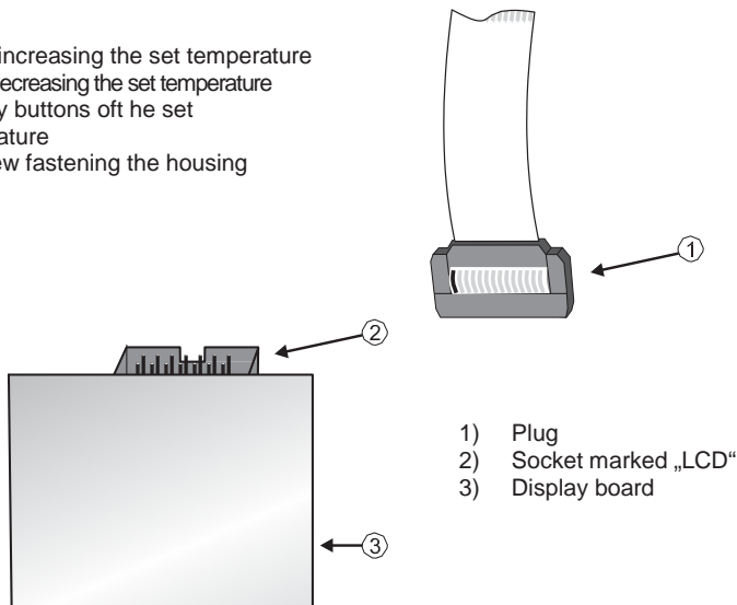
Fig. 2. Display board with ribbon cable
