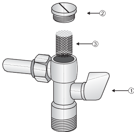
Abb. 5. Control valve with the filter
